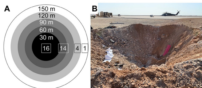
Figure 3 Proximity of our cohort to theatre ballistic missile (TBM) explosion blast radius. (A) Bull's eye diagram showing our cohorts closest distance to an exploding TBM (in 30 m intervals). Note: many individuals were exposed to multiple exploding TBMs, we display the closest distance. Sixteen individuals were within 0–30 m proximity, 14 were within 31–60 m, 4 were within 91–120 m and 1 was within 121–150 m. (B) Large hole left in the ground created by an exploded TBM ballistic missile. Image courtesy of Alan Johnson.
